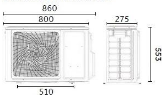
2U40S2SM1FA / 2U50S2SM1FA-3
